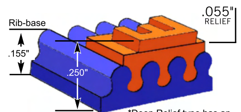
*Deep Relief type has an overall thickness of .270" and relief of .110".
